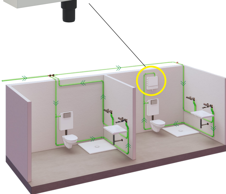
Hygiene Flush Box PRO, Figure 689 03 008
