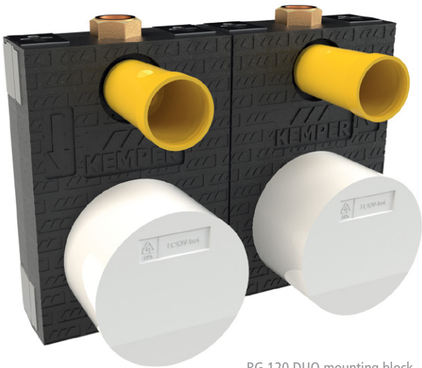
RG 120 DUO mounting block, Figure 854
