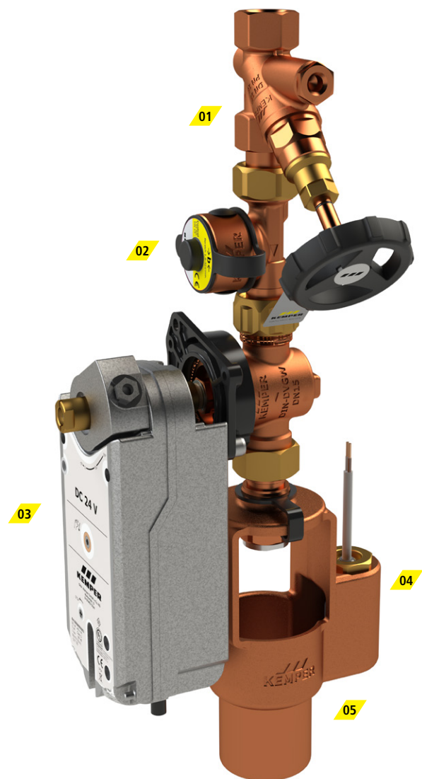
KHS Flush Point with CONTROL-PLUS, Figure 684 05
